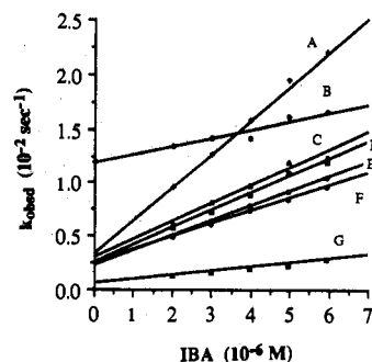
Figure 2. Dependence of k_{\text{obsd}} on IBA concentration in 0.2 mg mL -1 latex dispersions in pH 9.10, 5.0 mM TAPS, with 1.99 \times 10^{-5} M PNPDP: (A) TBAQ24; (B) HEDMAQ25; (C) TPAQ13; (D) TEAQ32; (E) TMAQ14; (F) TMAQ39; (G) TMAQ60.
